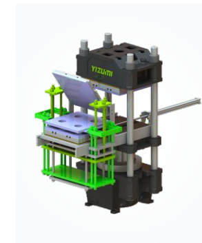
⑩ 3RT double lifter + mold tilting device
