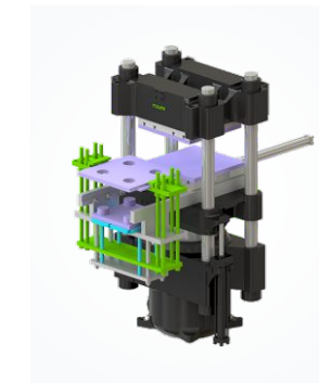
⑪ 3RT one lifter + one ejector
