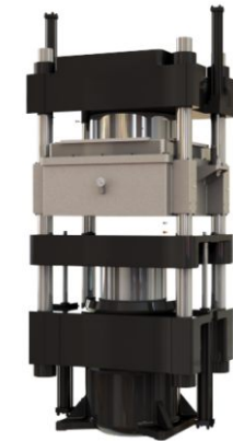
D6 Structure: 4-column 2-step upward closing with vacuum chamber; Features: Avoid air trapping, ideal for products with complex structure, no need for venting during injection, less flash.
