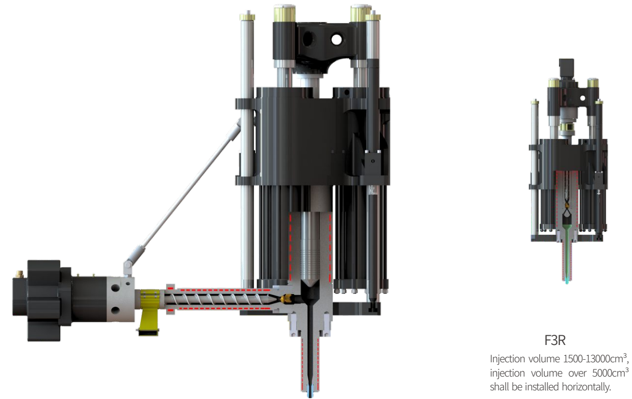
L3R Injection volume 1000-12000cm 3
